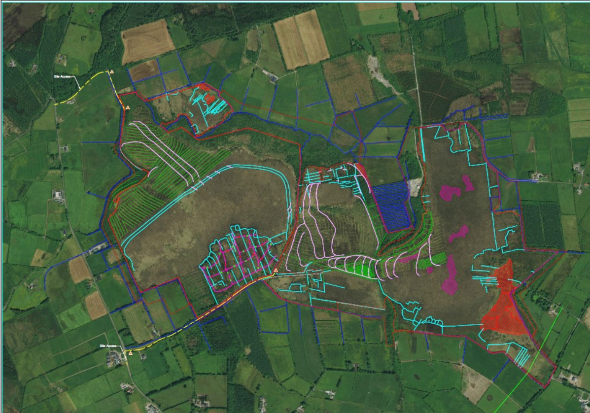
Figure 5.2 Contract Drawing showing the Restoration Works to be Constructed in Phase 1
