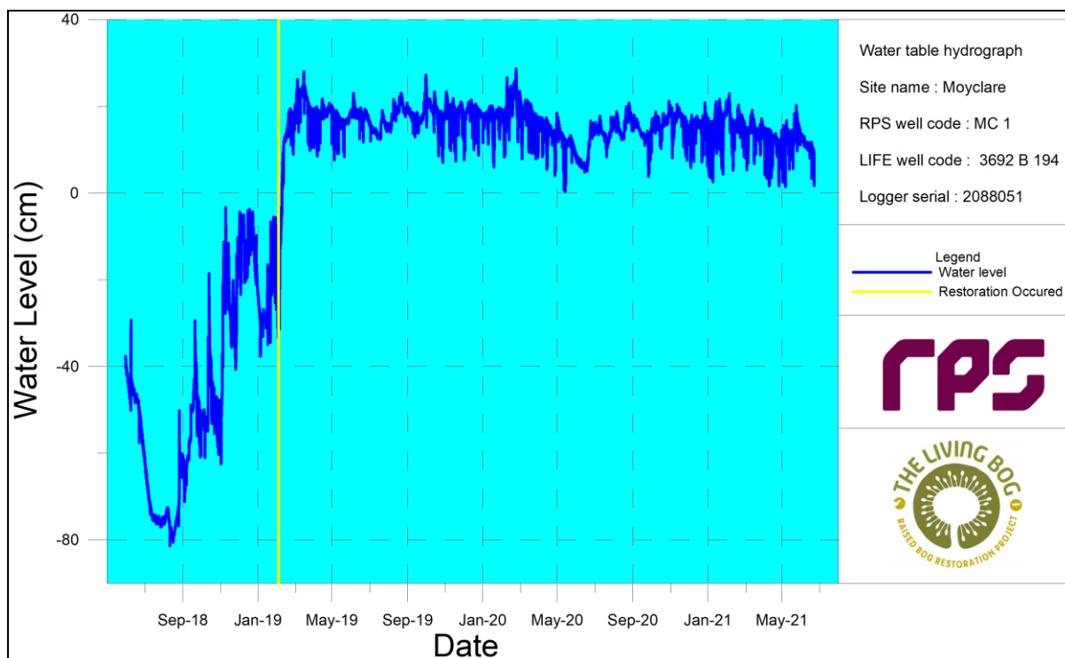
Figure 5.2 Example of hydrological response to drain blocking on cutover at Moyclare Bog SAC illustrating the water table rising from 80cm below ground to permanently remaining above ground surface
