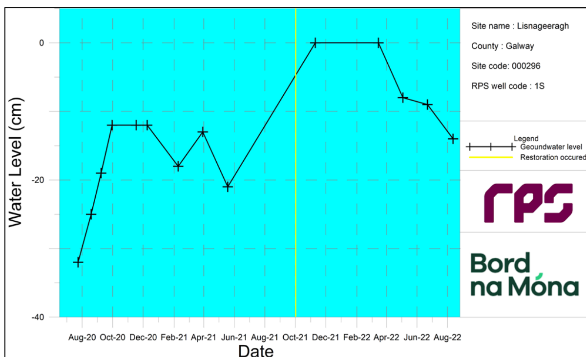
Figure 5.7 Example of Piezometer readings at Lisnageeragh Bog and Ballinastack Turlough SAC showing pre and post works water levels
