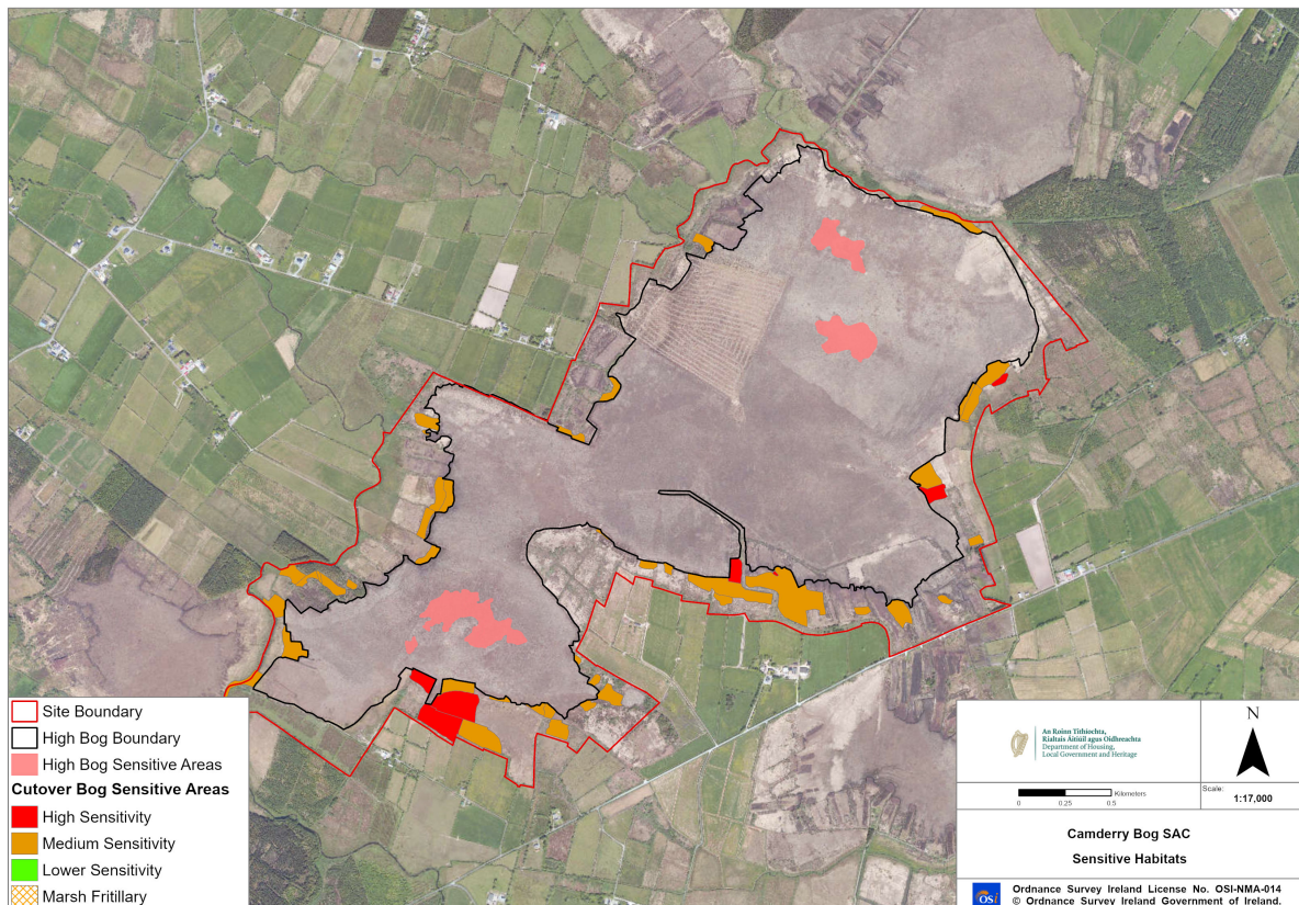
Figure 5.3 Sensitive habitats mapped at Camderry Bog SAC
