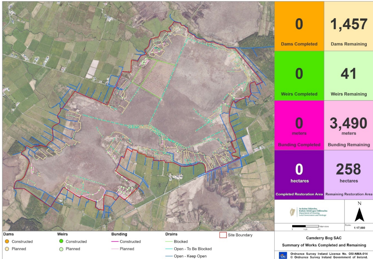
Figure 5.5 Summary of Works (all Phases) completed to date and Works remaining
