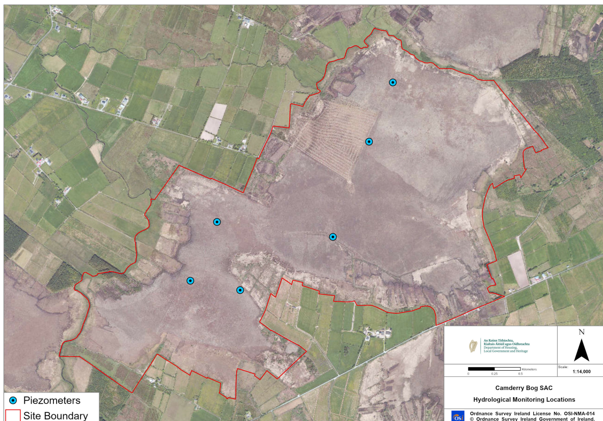
Figure 5.1 Location of hydrological monitoring network at Camderry Bog
