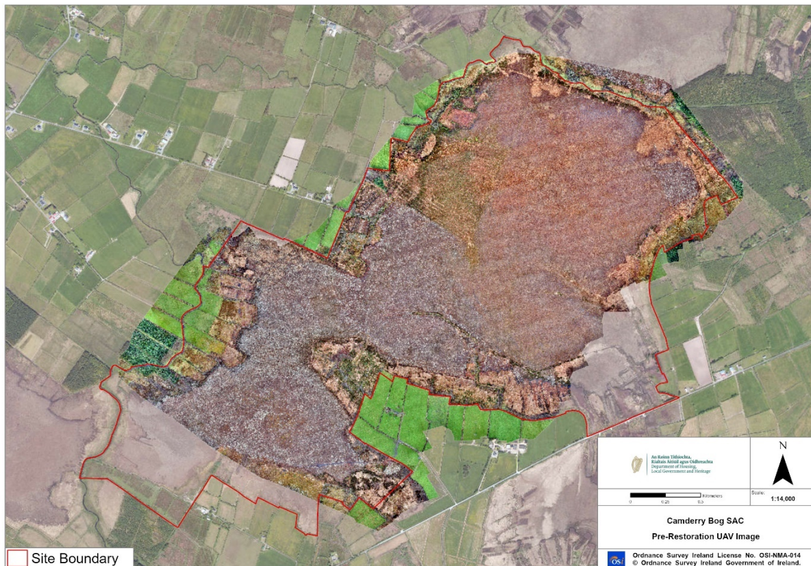
Figure 5.4 Pre-Restoration UAV Imagery of Camderry Bog
