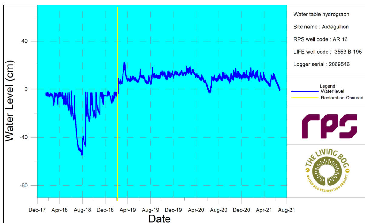
Figure 5.2 Example hydrography from the cutover at Ardagullion Bog SAC illustrating the significant impact of the marginal dam in bringing the water table above the ground surface
